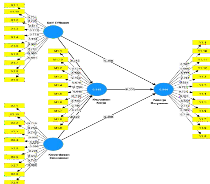
Gambar 2. Hasil Outer Loading 1
