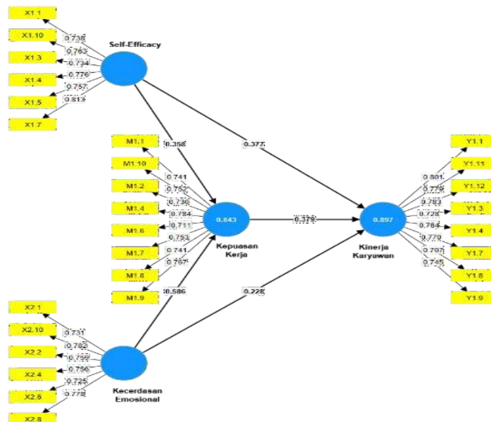
Gambar 3. Hasil Outer Loading 2
